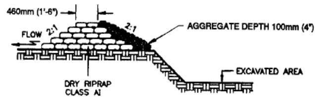
CROSS-SECTION B-B
