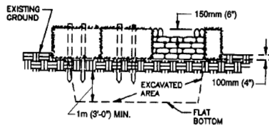
CROSS-SECTION A-A
